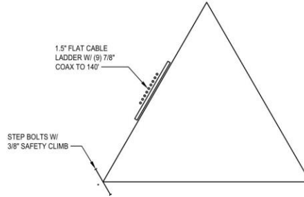
COAX LAYOUT
