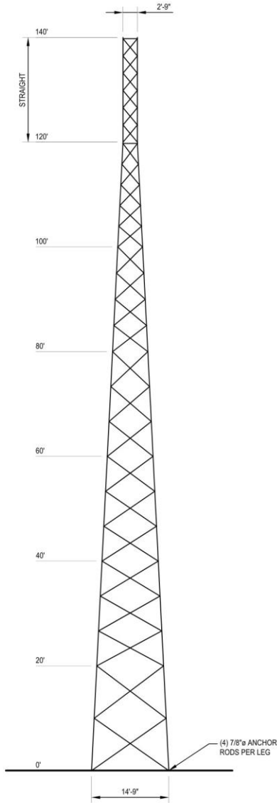
TOWER ELEVATION
