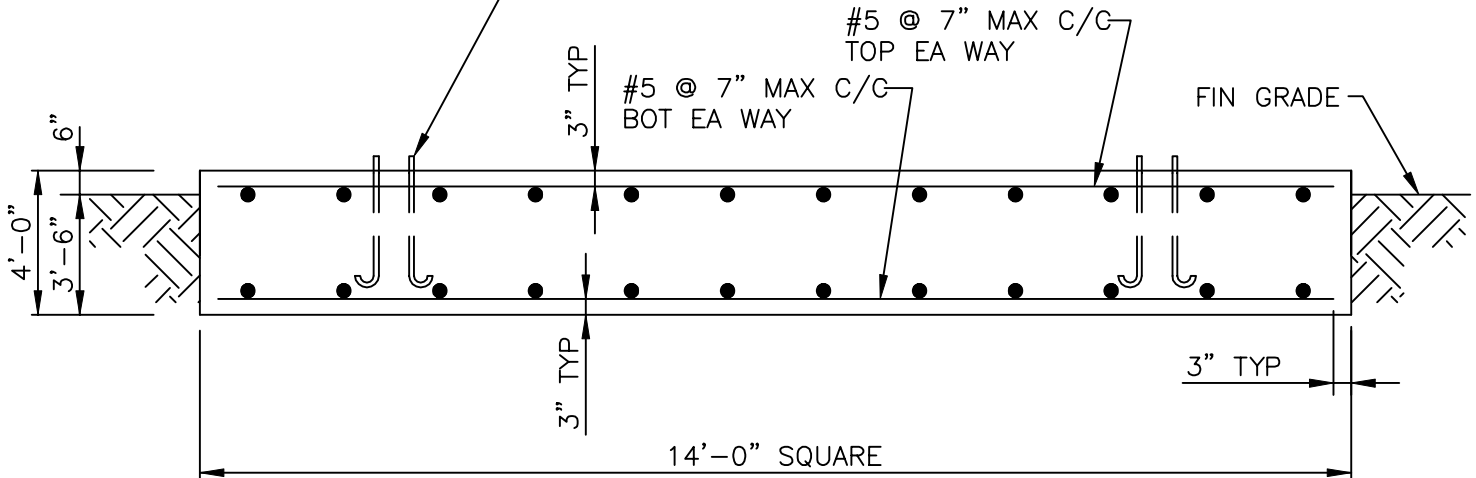
MAT FOUNDATION
